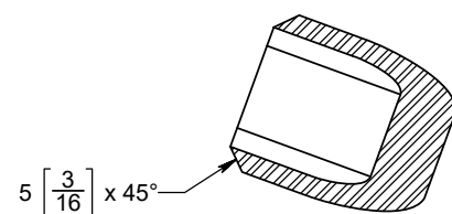
SECTION H-H
